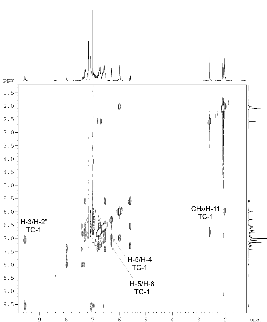
FIGURE 3 2D-Rosy of CF-1 after UV irradiation.
