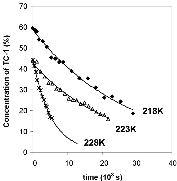
FIGURE 4 Thermal evolution of TC-1 .
