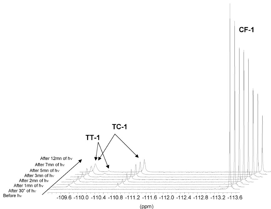
FIGURE 1 ^{19}\text{F} NMR spectra recorded during UV irradiation at 203 K.
