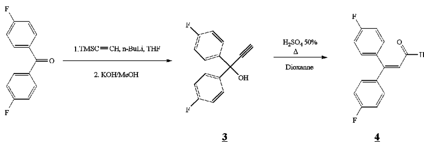
SCHEME 1 General synthesis of 3,3-di-(4'-fluorophenyl)prop-2-enal, 4 .
