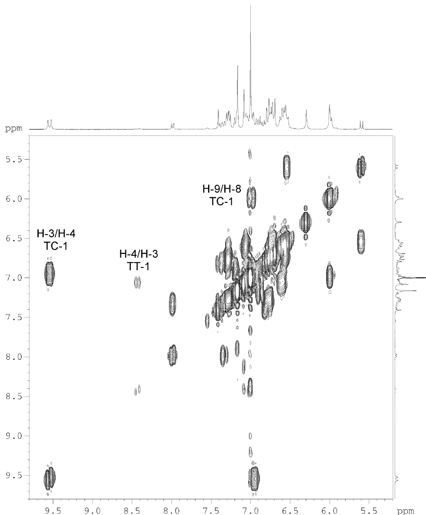
FIGURE 2 2D-Cosy of CF-1 after UV irradiation.
