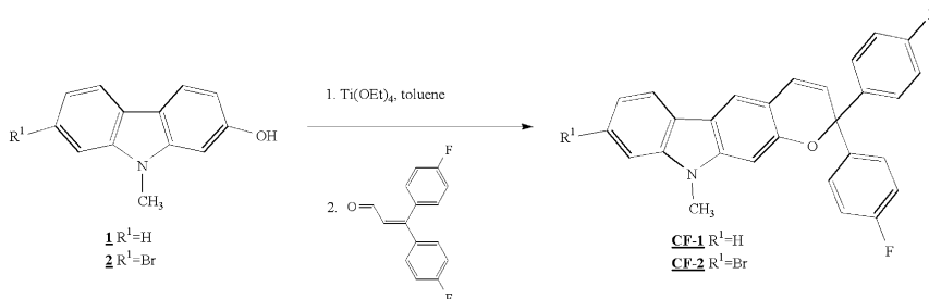
SCHEME 2 General synthesis of [indole]benzopyrans CF-1 and CF-2 .
